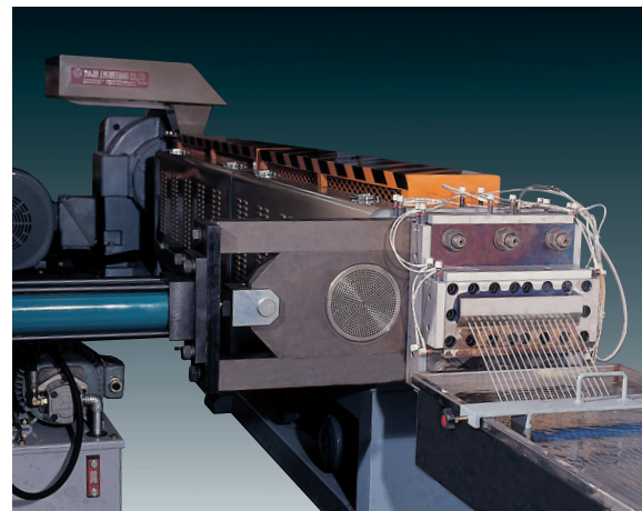
Semi-Auto Hydraulic Screen Changer
