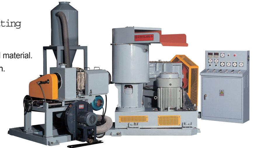
Hot Dies Face-Cutting Type by Air-Cooling
